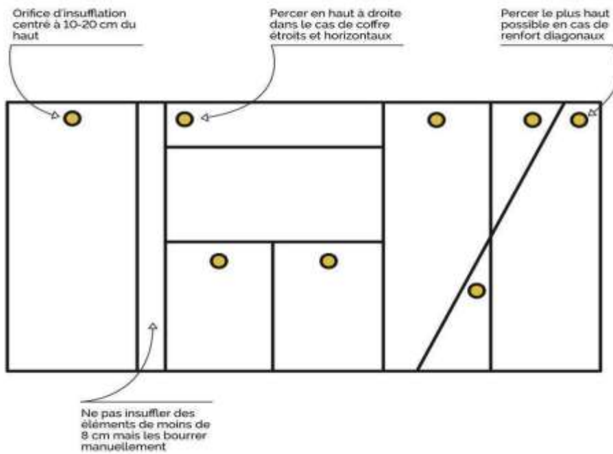
Figure 5: Emplacement des orifices d'insufflation
